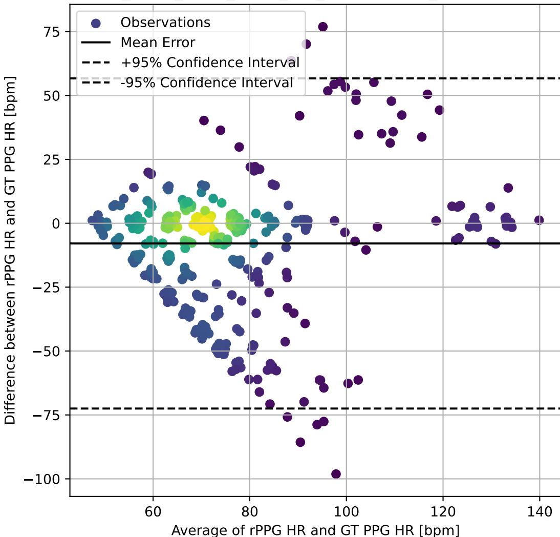
UBFC_UBFC_PURE_tscan_FFT_BlandAltman_DifferencePlot
