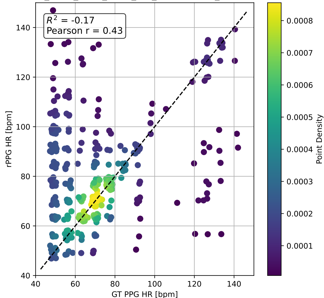
UBFC_UBFC_PURE_tscan_FFT_BlandAltman_ScatterPlot
