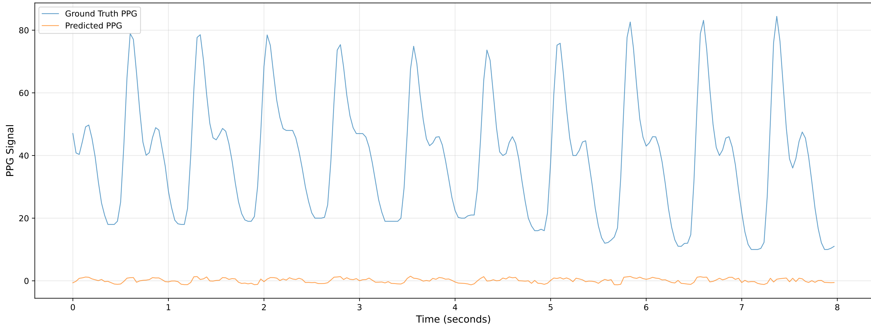
Video 1001 - Chunk 7 - Predicted vs Ground Truth PPG
