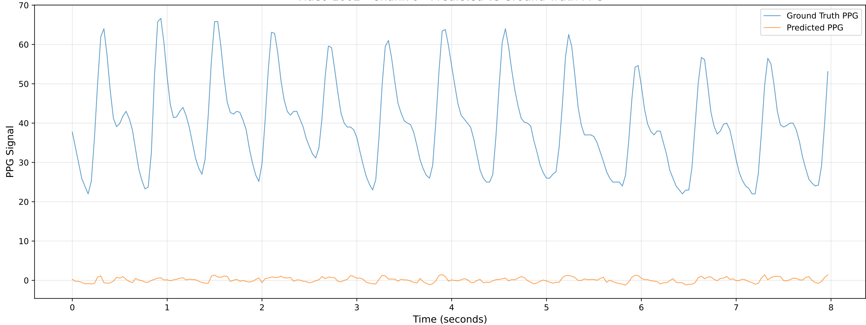
Video 1002 - Chunk 6 - Predicted vs Ground Truth PPG
