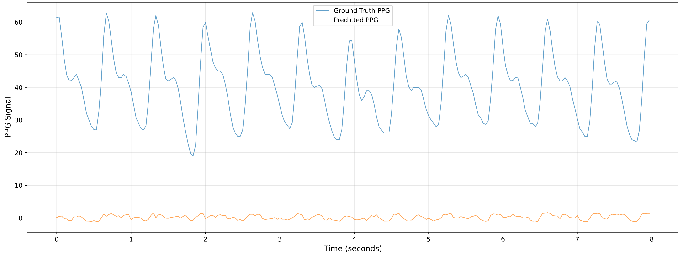
Video 1002 - Chunk 7 - Predicted vs Ground Truth PPG
