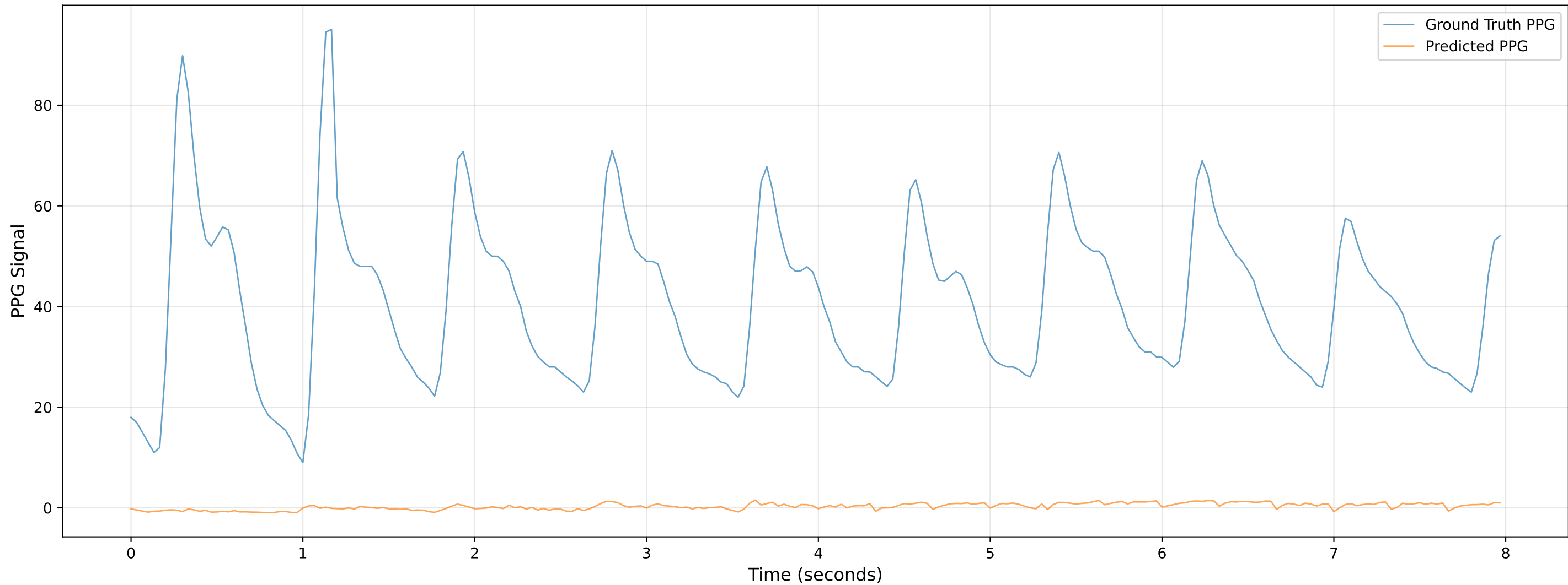
Video 1003 - Chunk 2 - Predicted vs Ground Truth PPG
