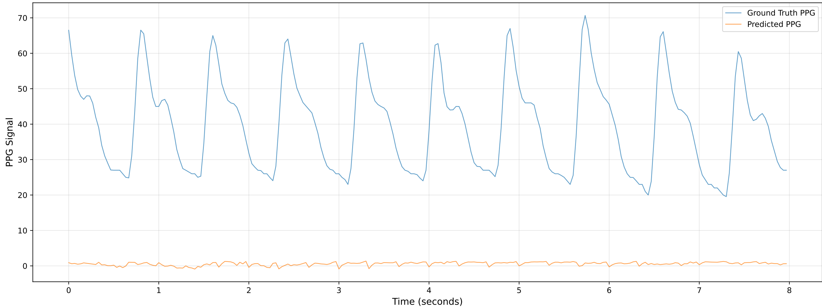
Video 1003 - Chunk 5 - Predicted vs Ground Truth PPG
