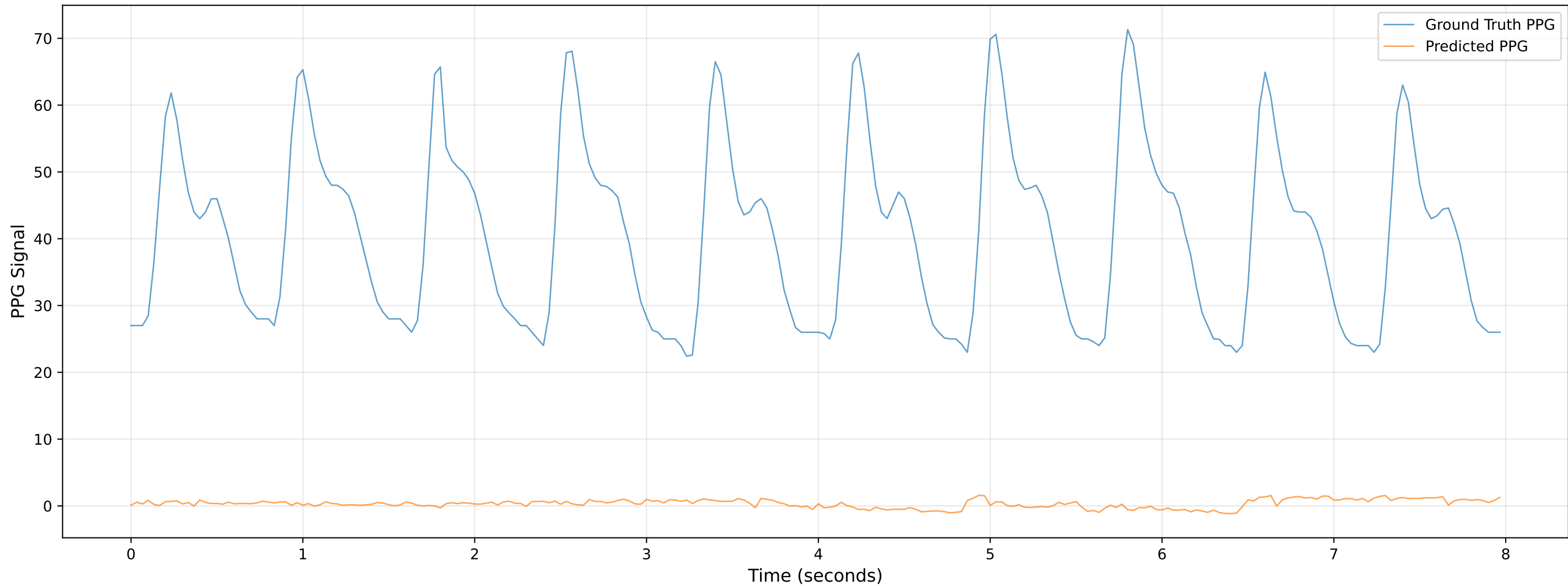
Video 1003 - Chunk 6 - Predicted vs Ground Truth PPG
