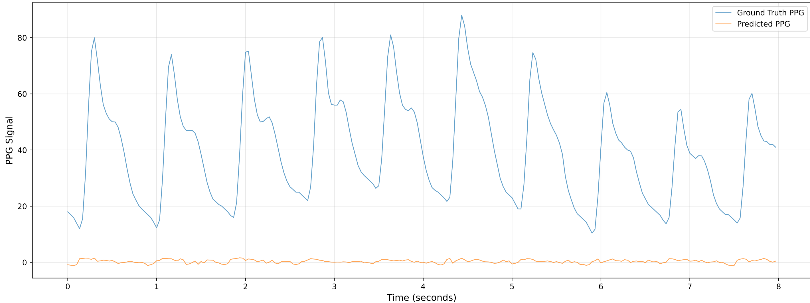
Video 1005 - Chunk 2 - Predicted vs Ground Truth PPG
