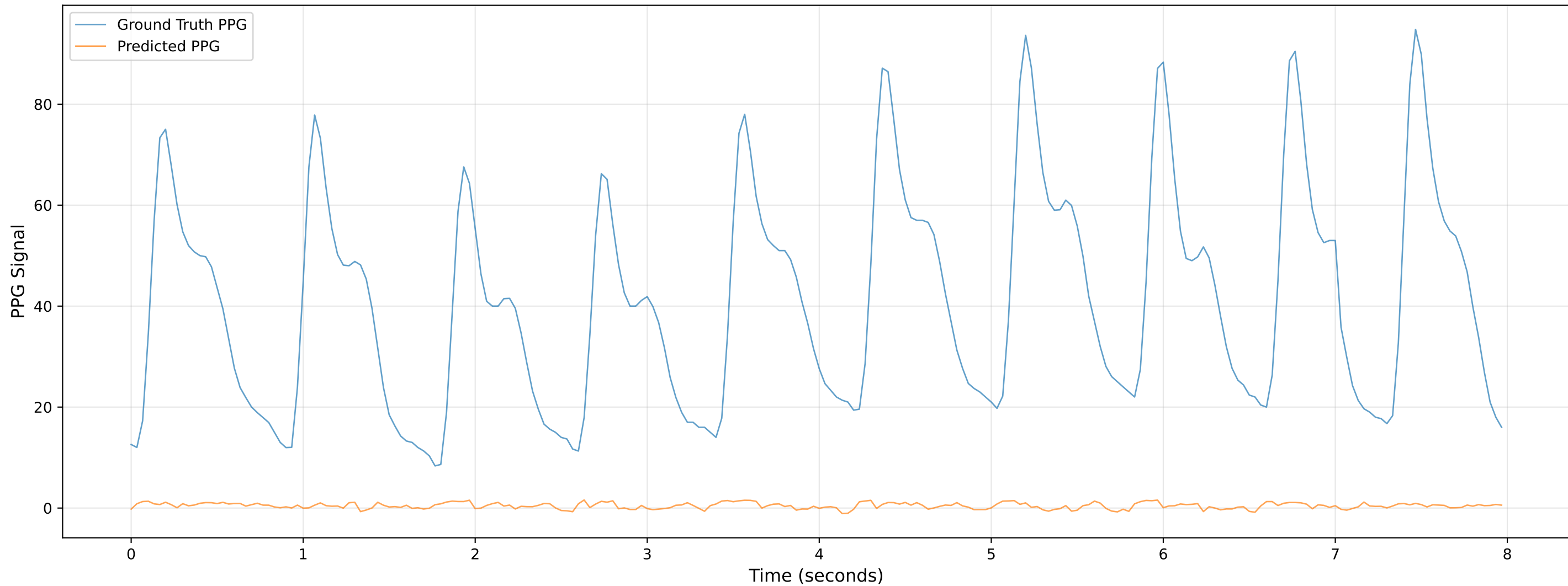
Video 1005 - Chunk 6 - Predicted vs Ground Truth PPG
