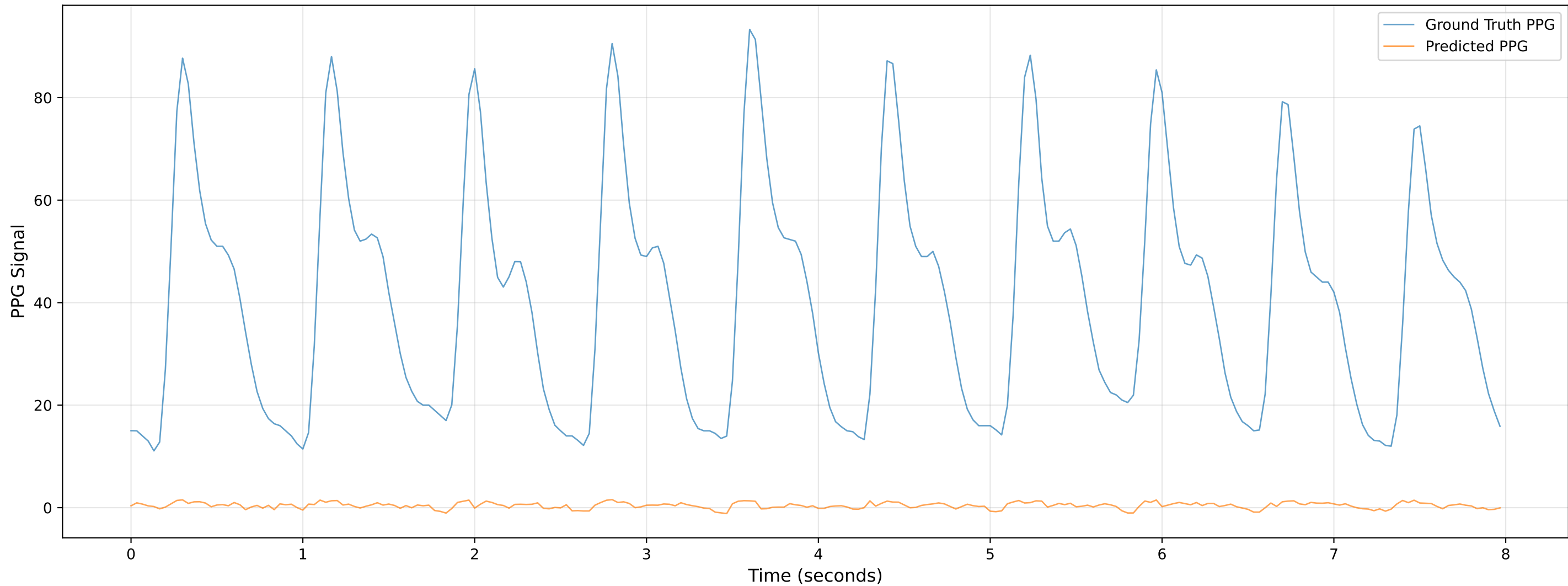
Video 1005 - Chunk 7 - Predicted vs Ground Truth PPG
