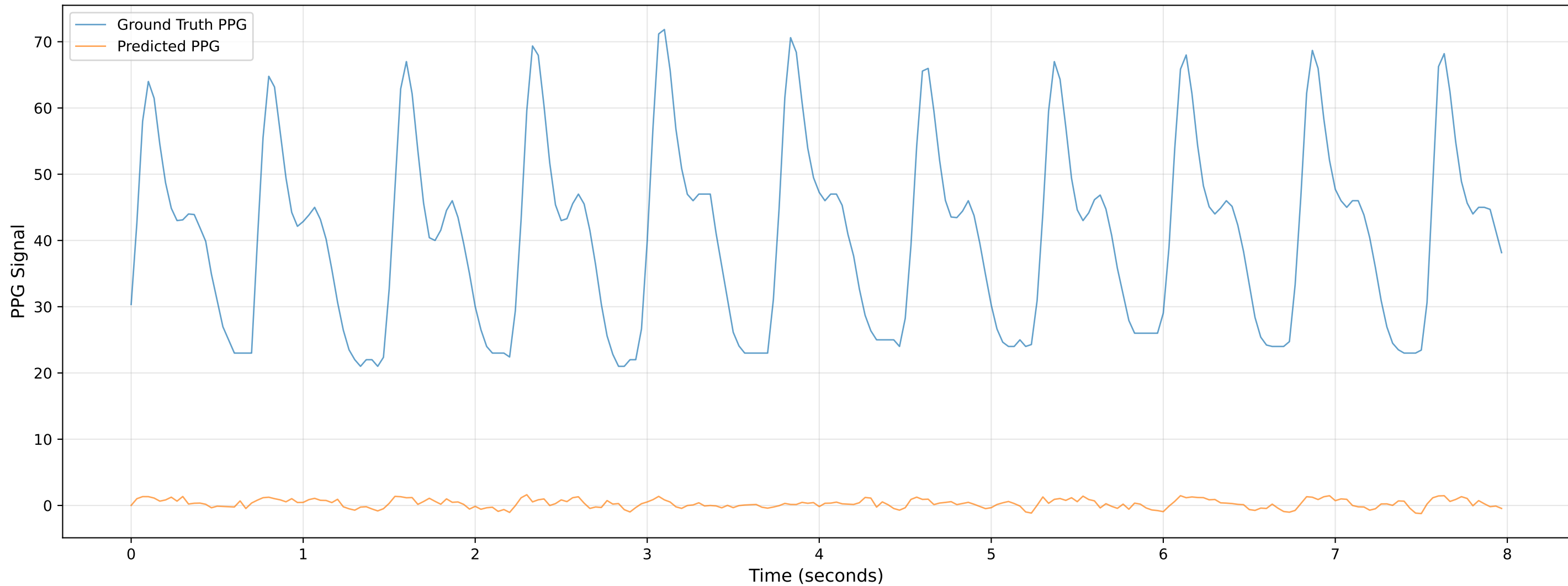
Video 1006 - Chunk 5 - Predicted vs Ground Truth PPG
