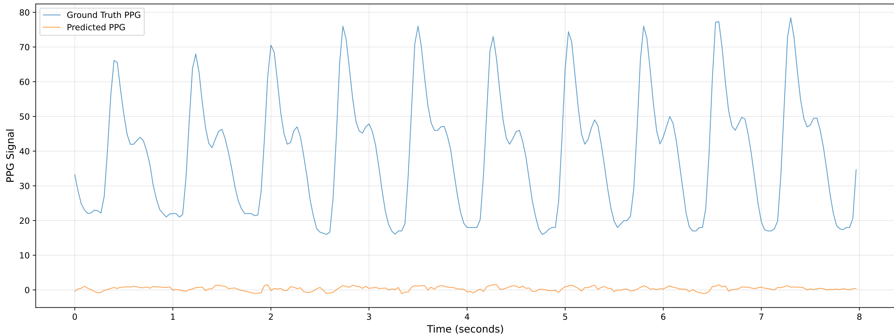
Video 1006 - Chunk 6 - Predicted vs Ground Truth PPG
