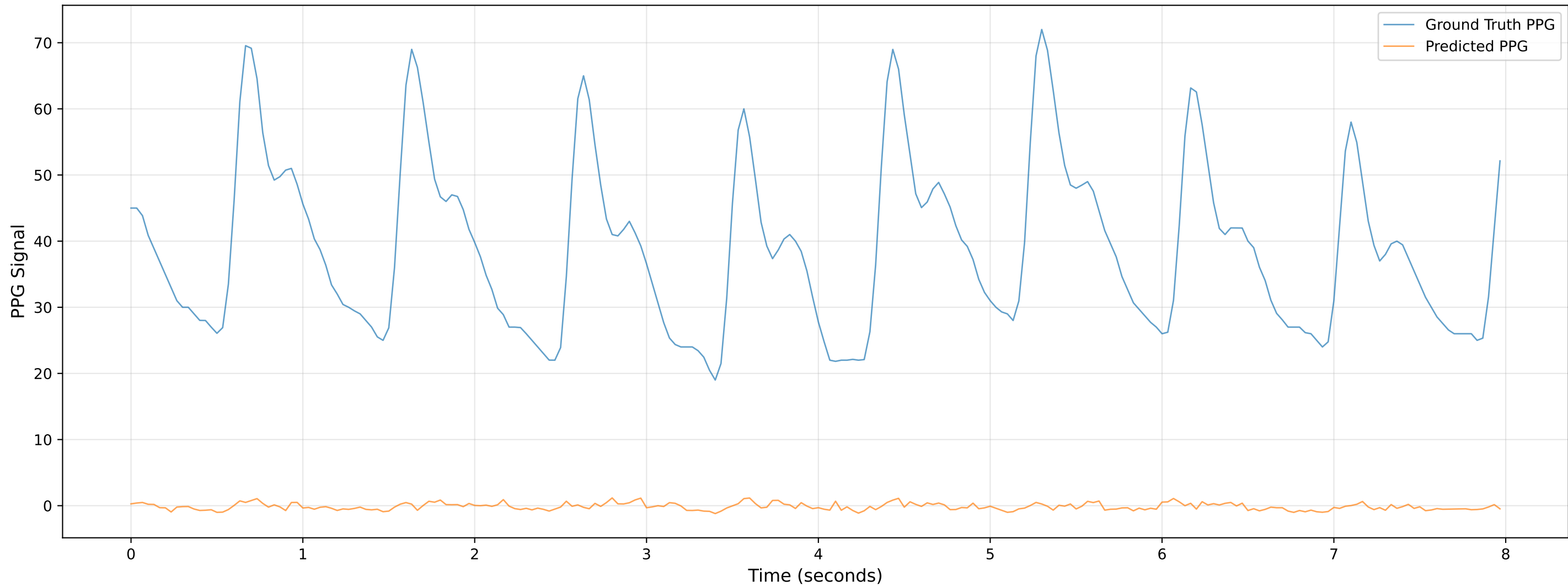
Video 101 - Chunk 2 - Predicted vs Ground Truth PPG
