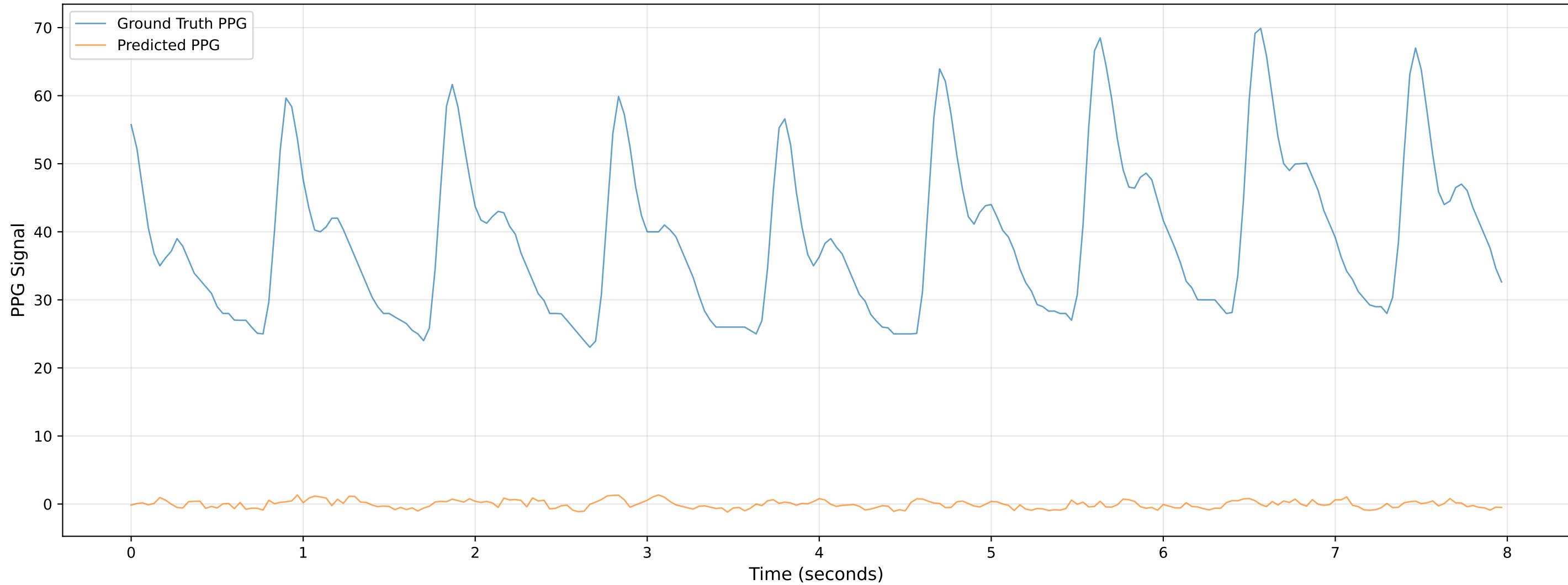
Video 101 - Chunk 3 - Predicted vs Ground Truth PPG
