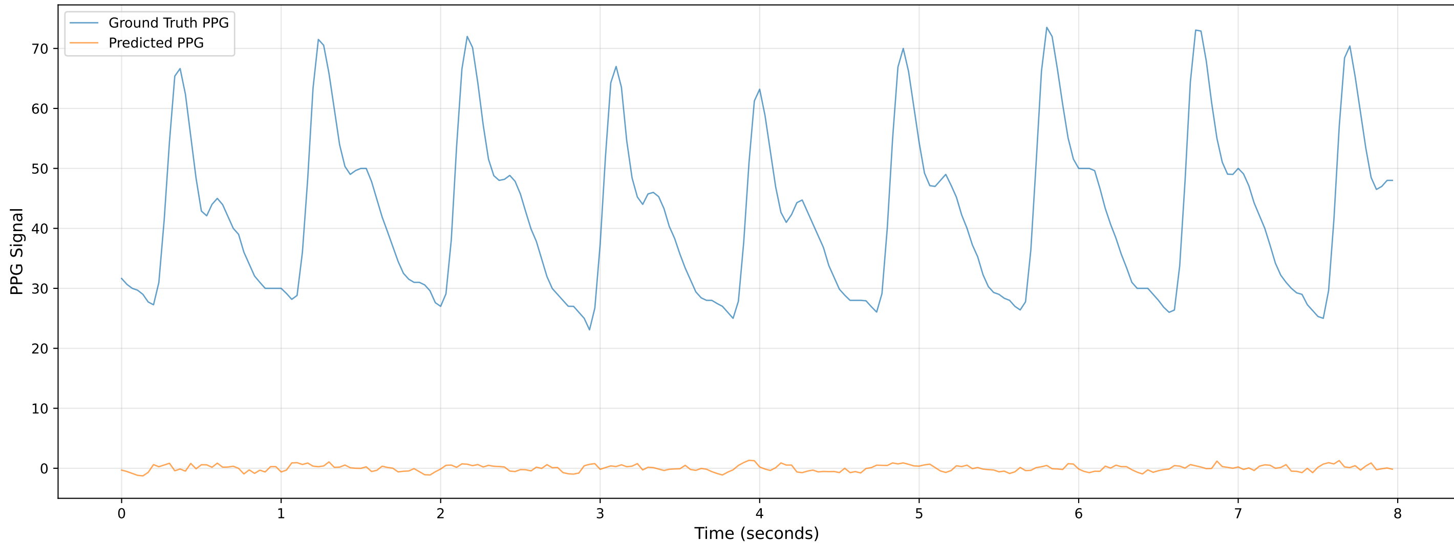
Video 101 - Chunk 4 - Predicted vs Ground Truth PPG
