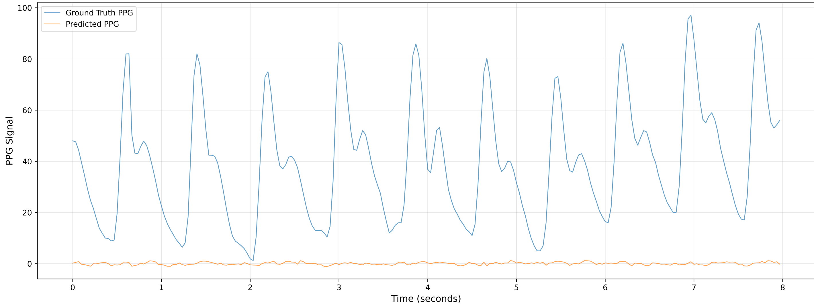
Video 102 - Chunk 6 - Predicted vs Ground Truth PPG
