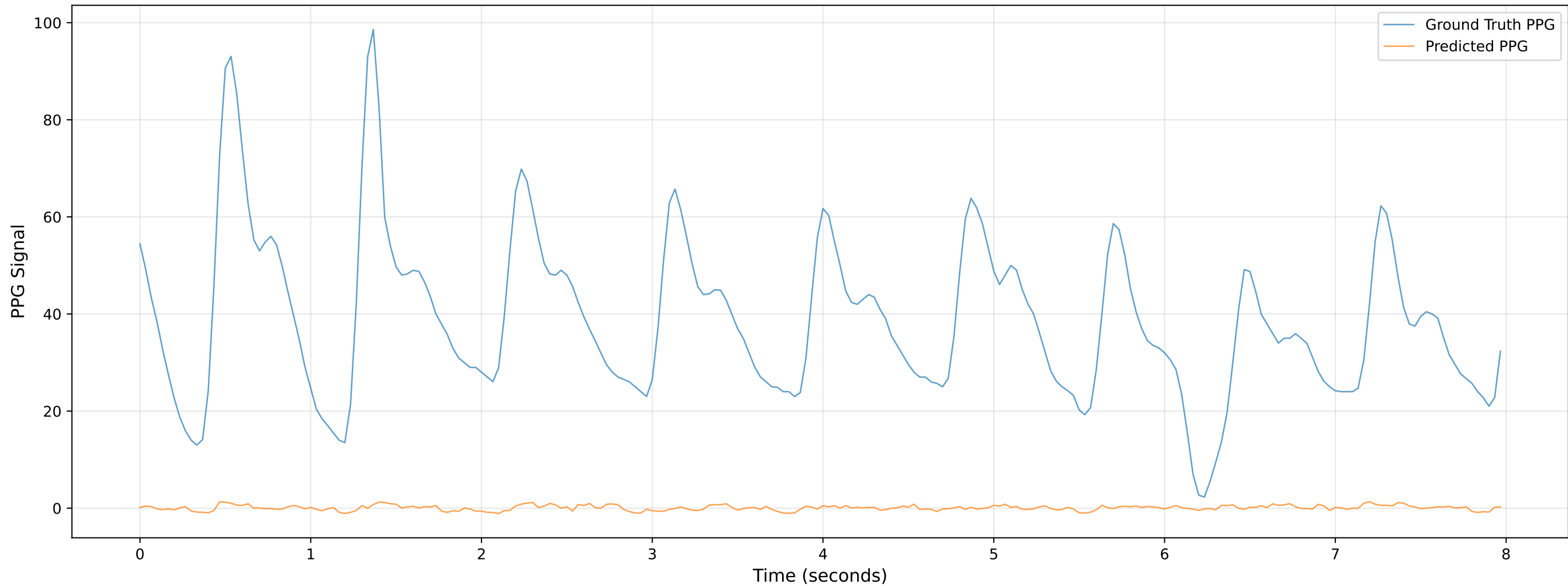
Video 102 - Chunk 7 - Predicted vs Ground Truth PPG
