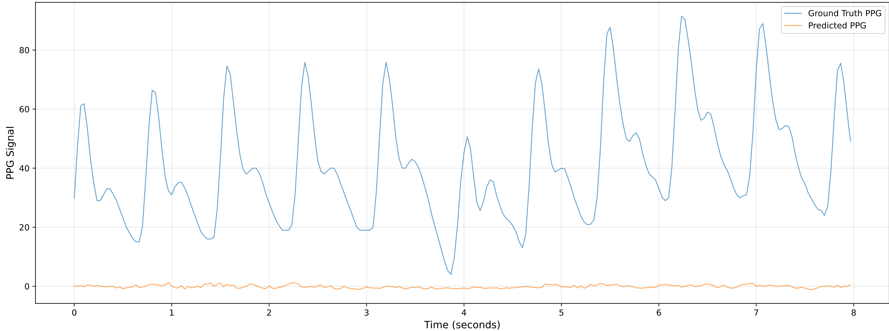
Video 103 - Chunk 1 - Predicted vs Ground Truth PPG
