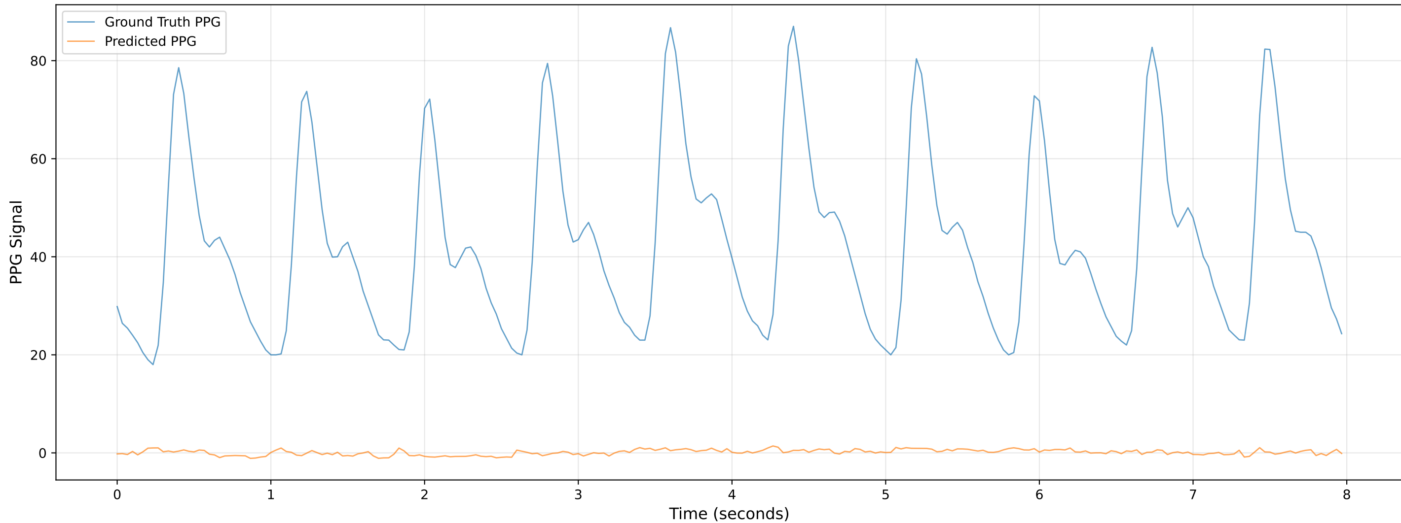
Video 103 - Chunk 6 - Predicted vs Ground Truth PPG
