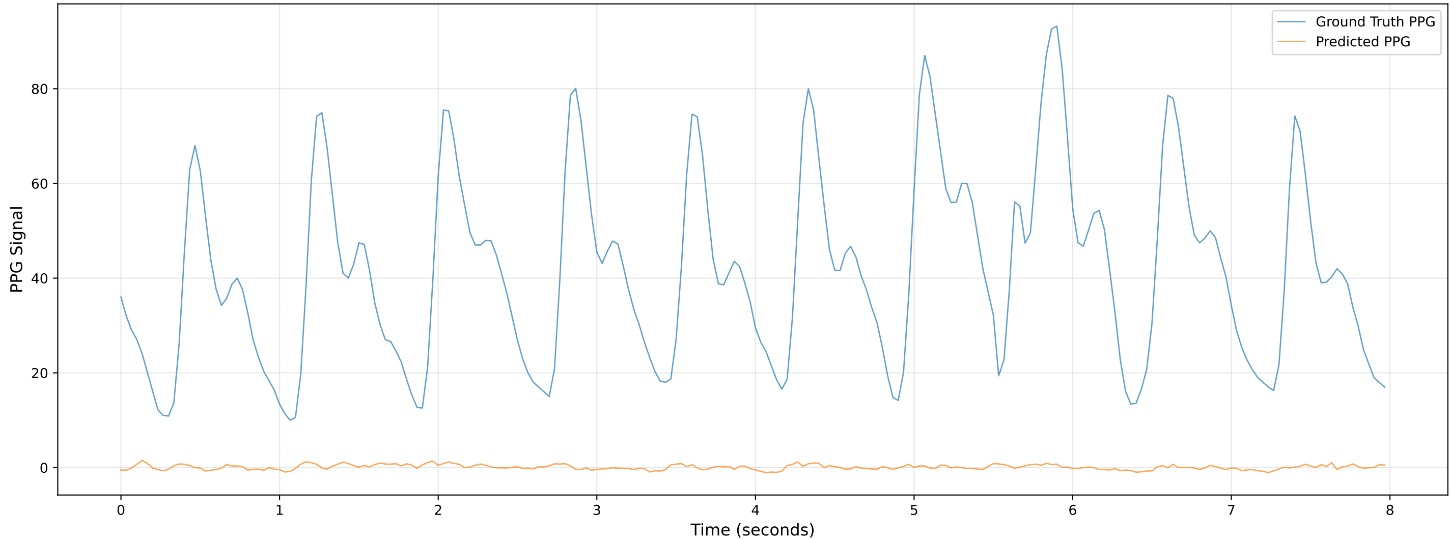
Video 104 - Chunk 0 - Predicted vs Ground Truth PPG
