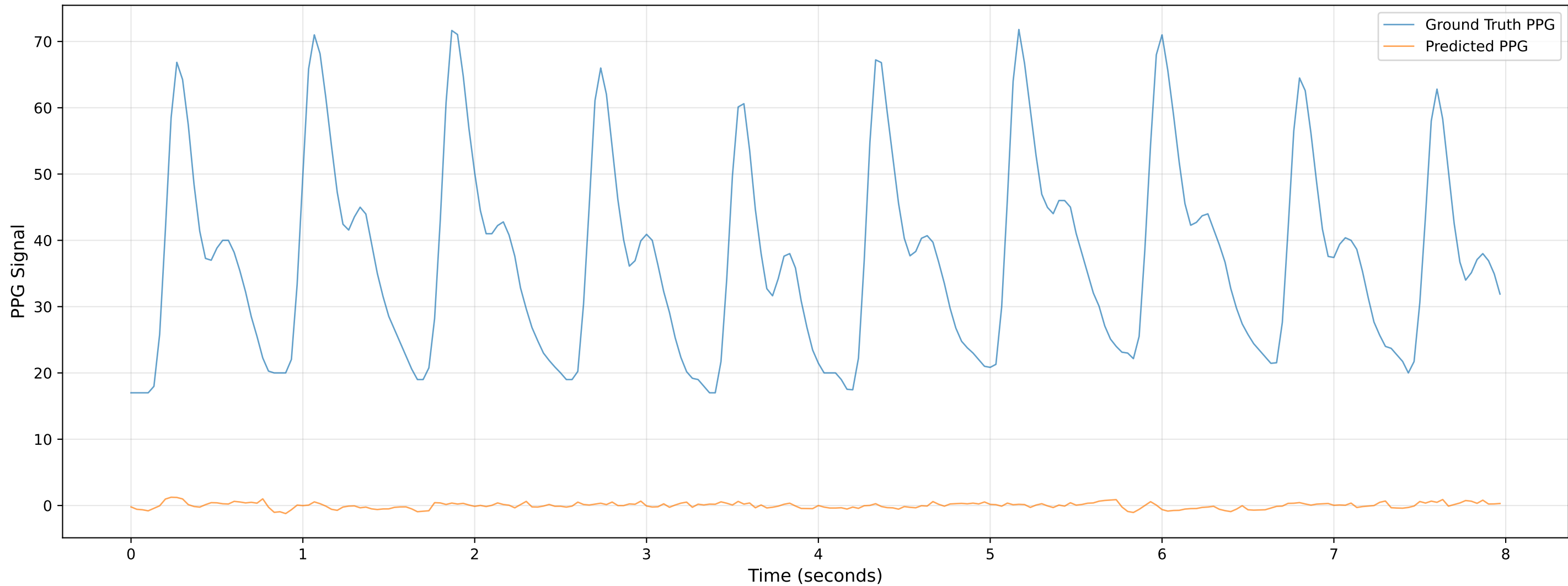
Video 104 - Chunk 2 - Predicted vs Ground Truth PPG
