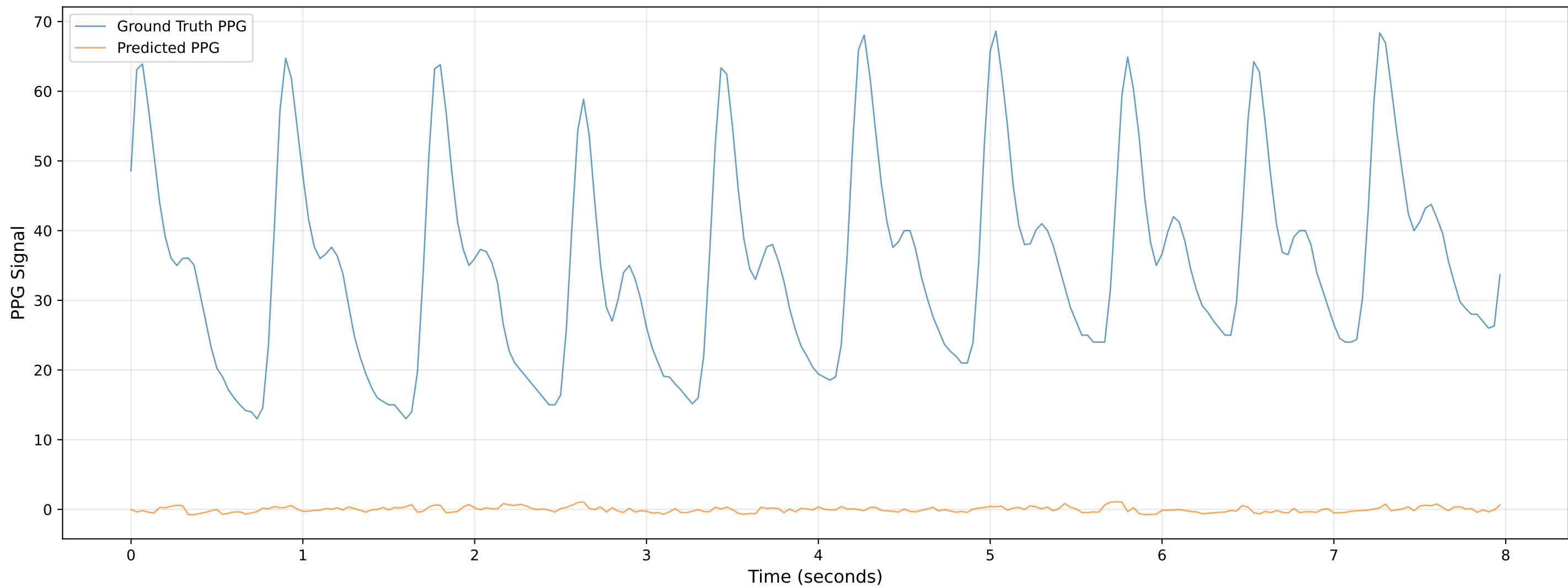
Video 104 - Chunk 5 - Predicted vs Ground Truth PPG
