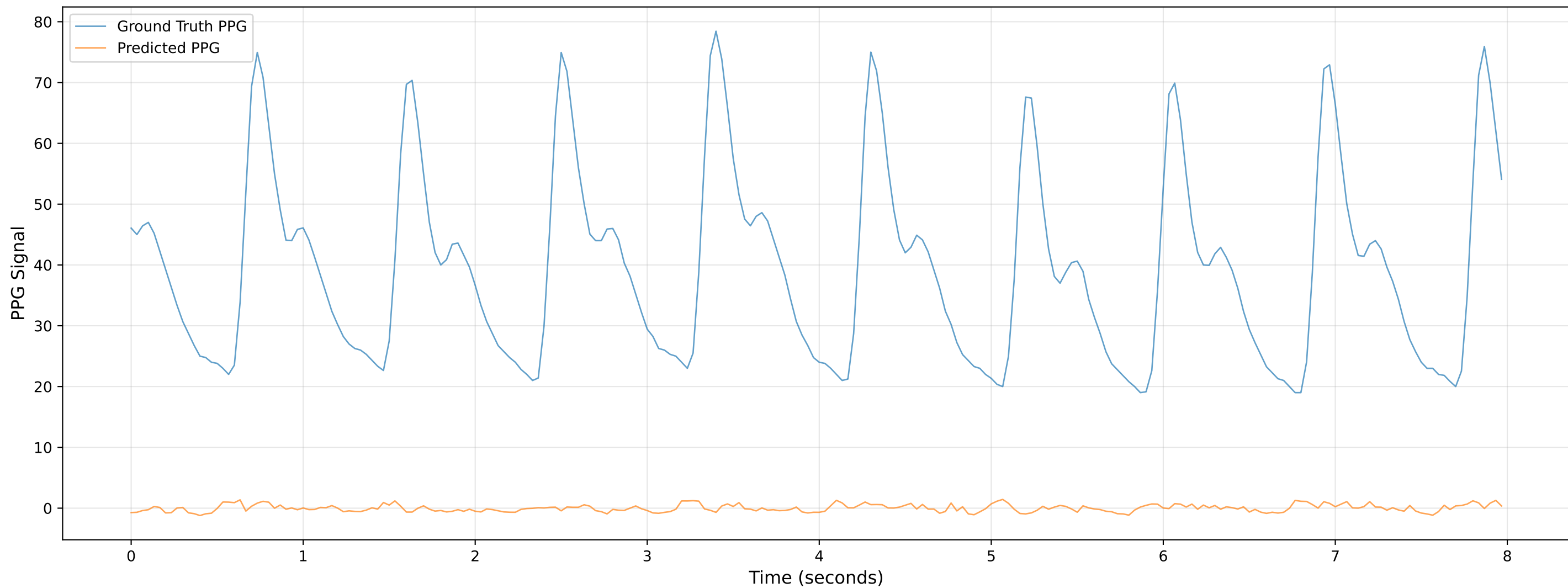
Video 105 - Chunk 3 - Predicted vs Ground Truth PPG
