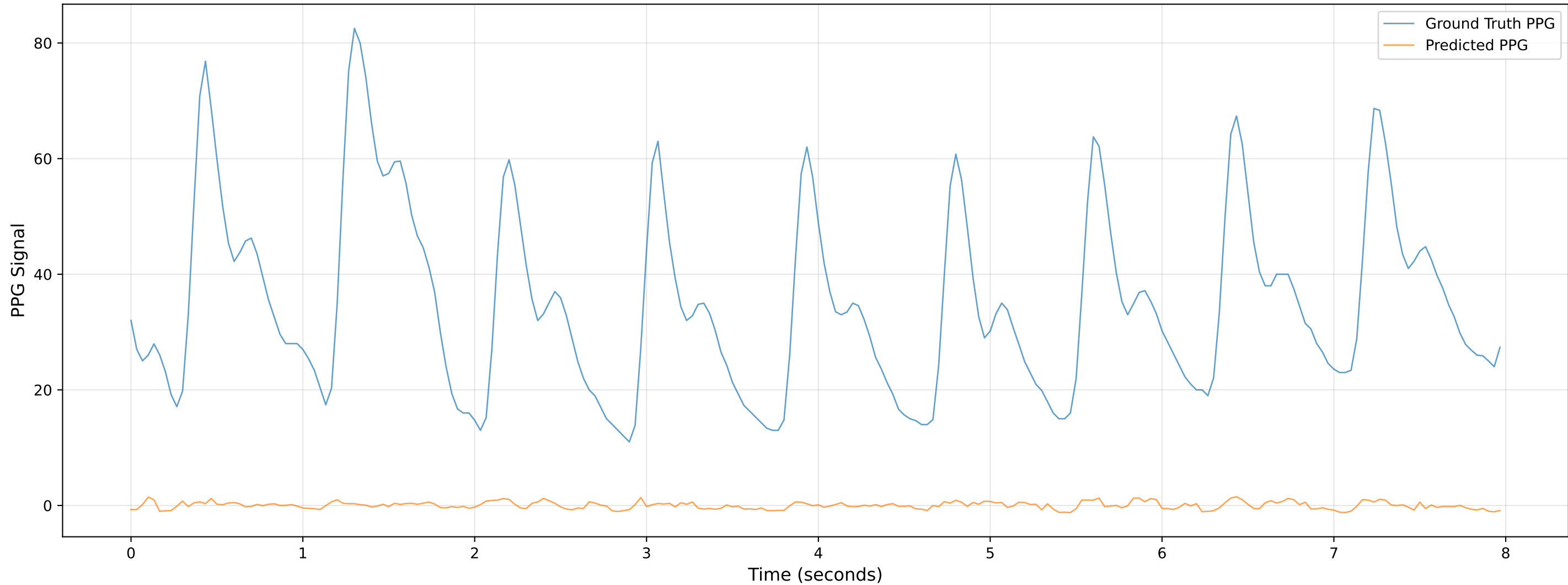
Video 106 - Chunk 0 - Predicted vs Ground Truth PPG
