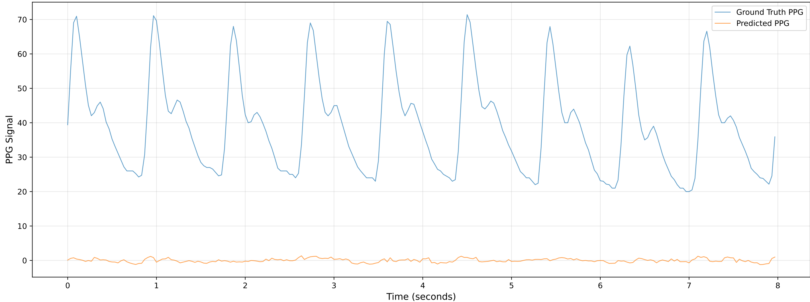
Video 106 - Chunk 1 - Predicted vs Ground Truth PPG
