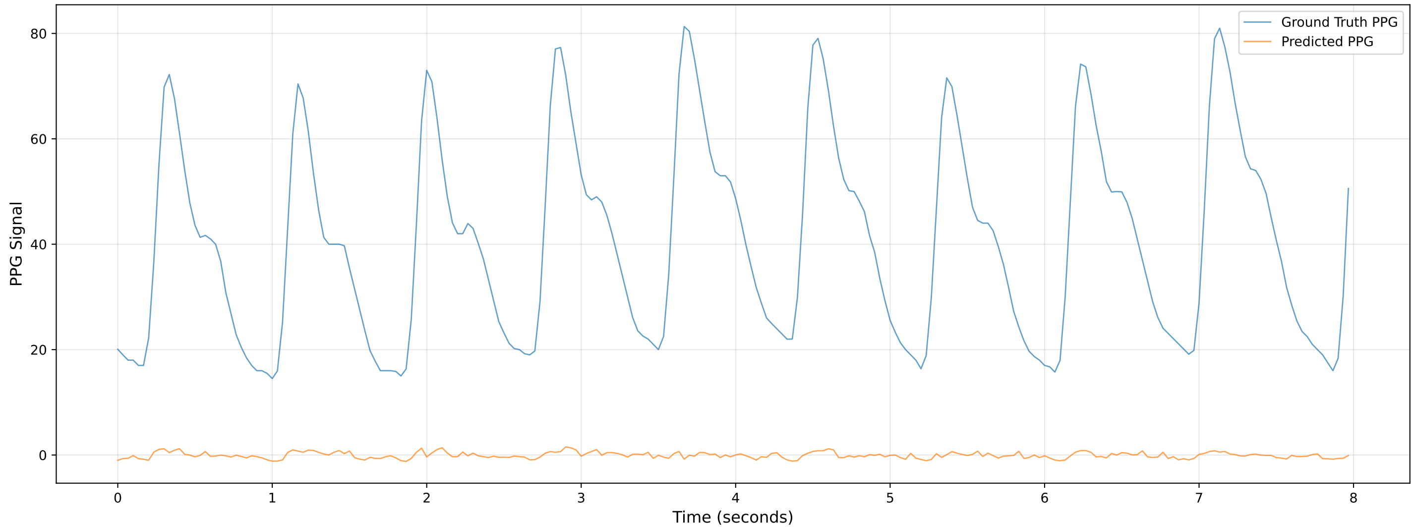
Video 201 - Chunk 2 - Predicted vs Ground Truth PPG
