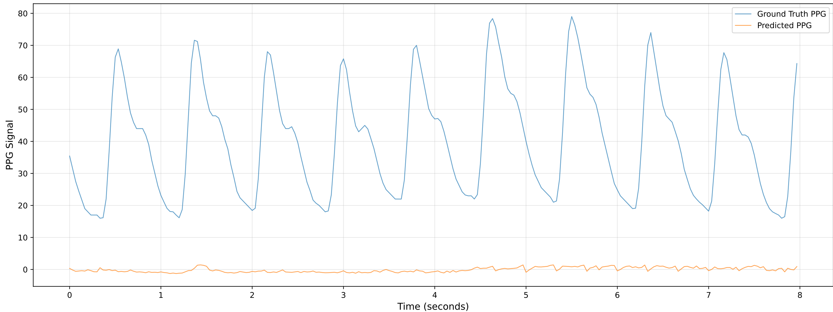
Video 203 - Chunk 2 - Predicted vs Ground Truth PPG
