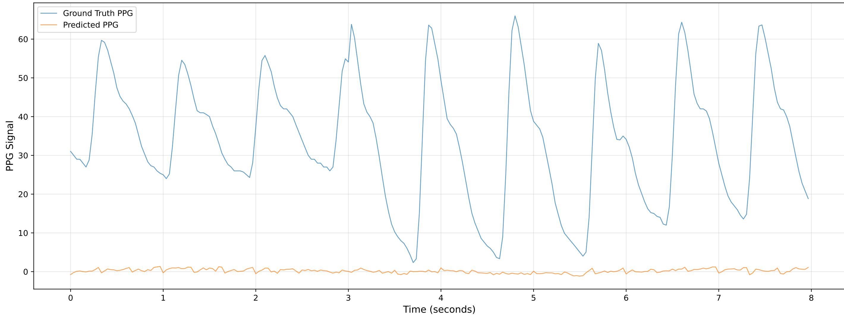
Video 204 - Chunk 5 - Predicted vs Ground Truth PPG
