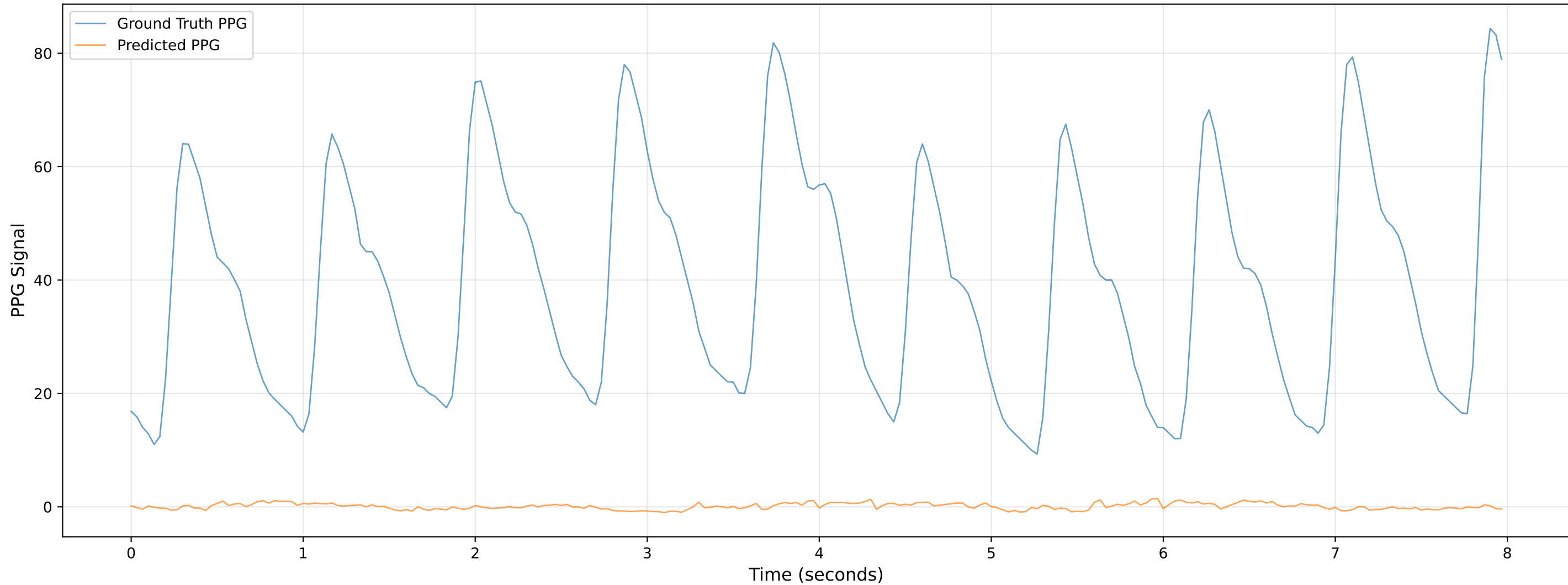
Video 204 - Chunk 6 - Predicted vs Ground Truth PPG
