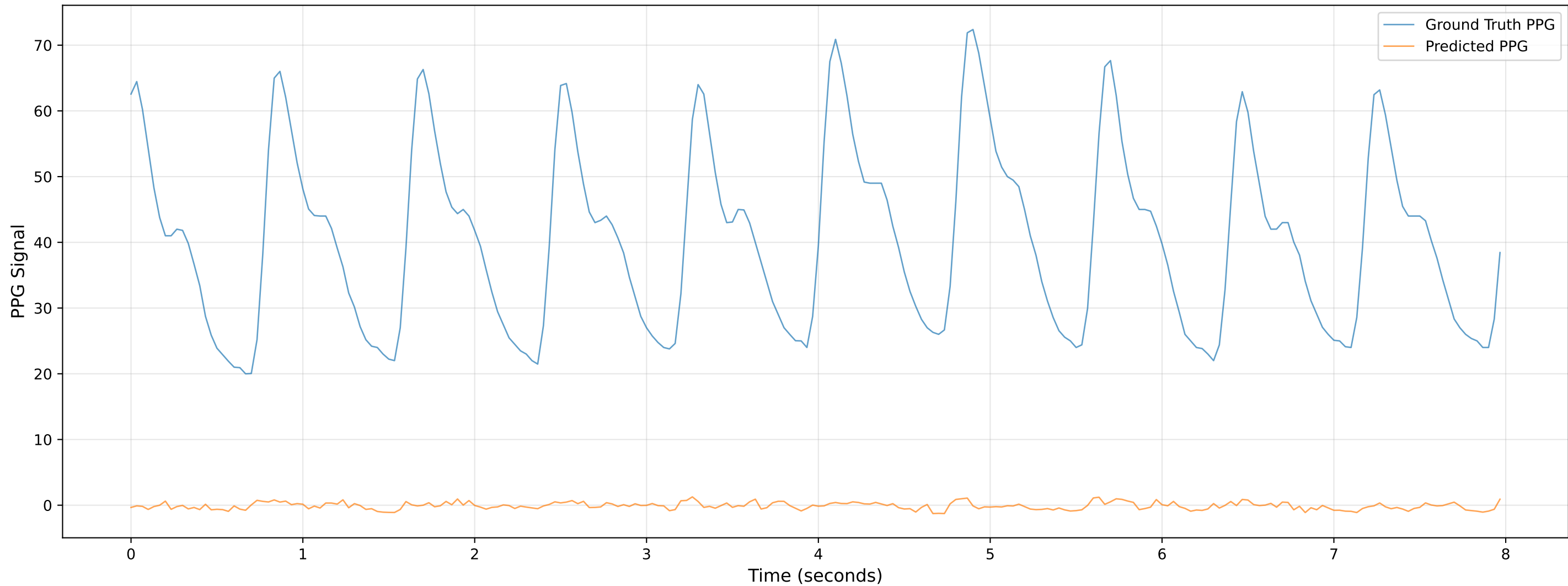
Video 206 - Chunk 1 - Predicted vs Ground Truth PPG
