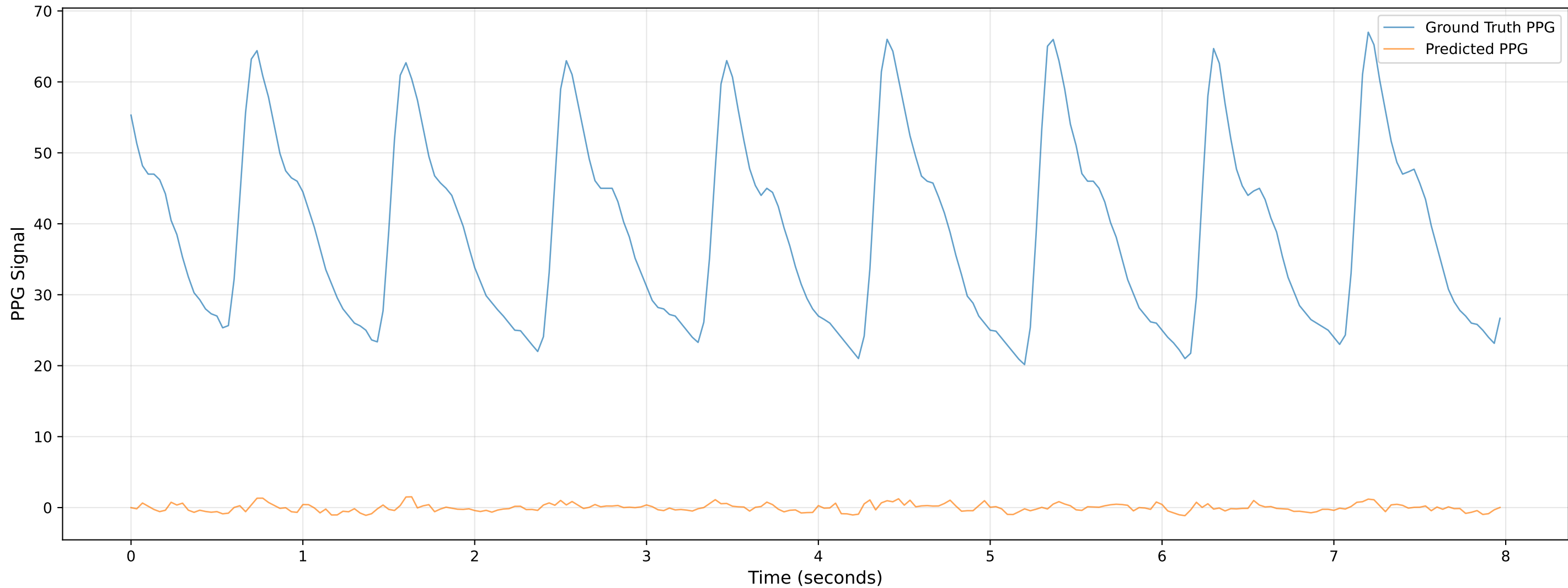
Video 206 - Chunk 3 - Predicted vs Ground Truth PPG
