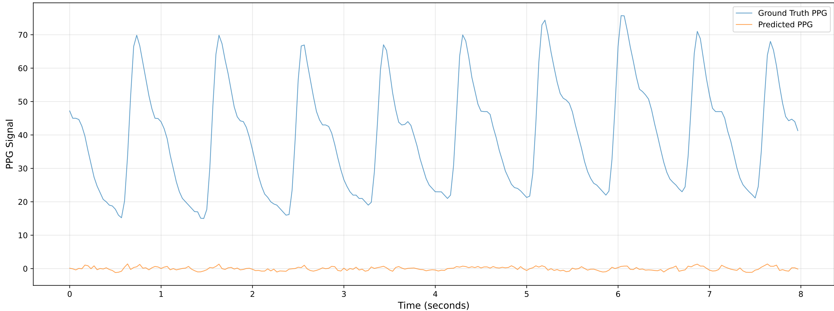
Video 206 - Chunk 5 - Predicted vs Ground Truth PPG
