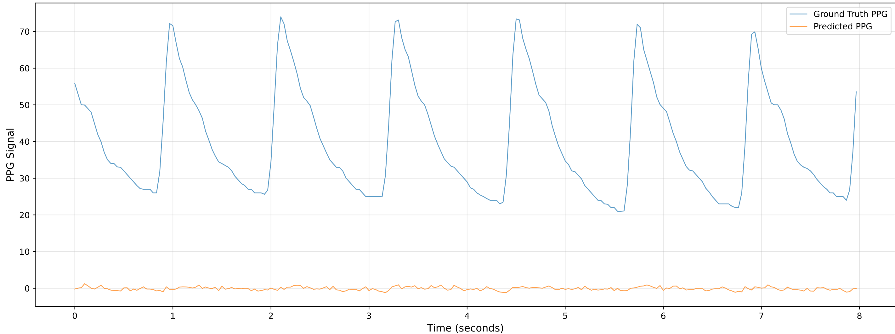
Video 301 - Chunk 1 - Predicted vs Ground Truth PPG
