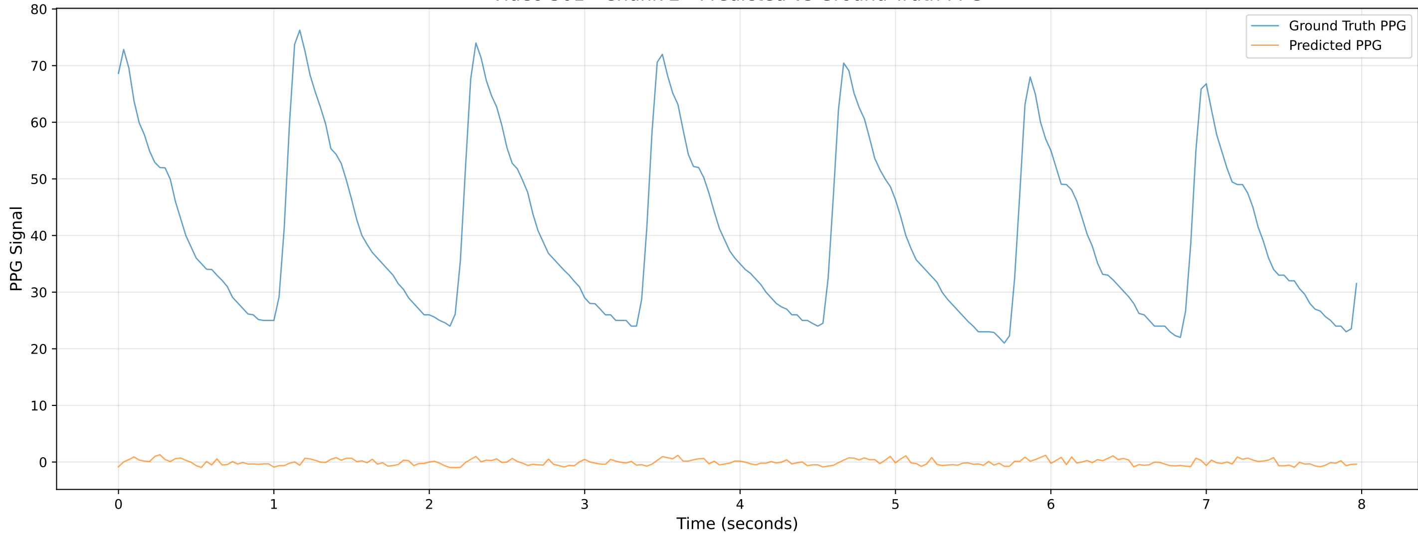
Video 301 - Chunk 2 - Predicted vs Ground Truth PPG
