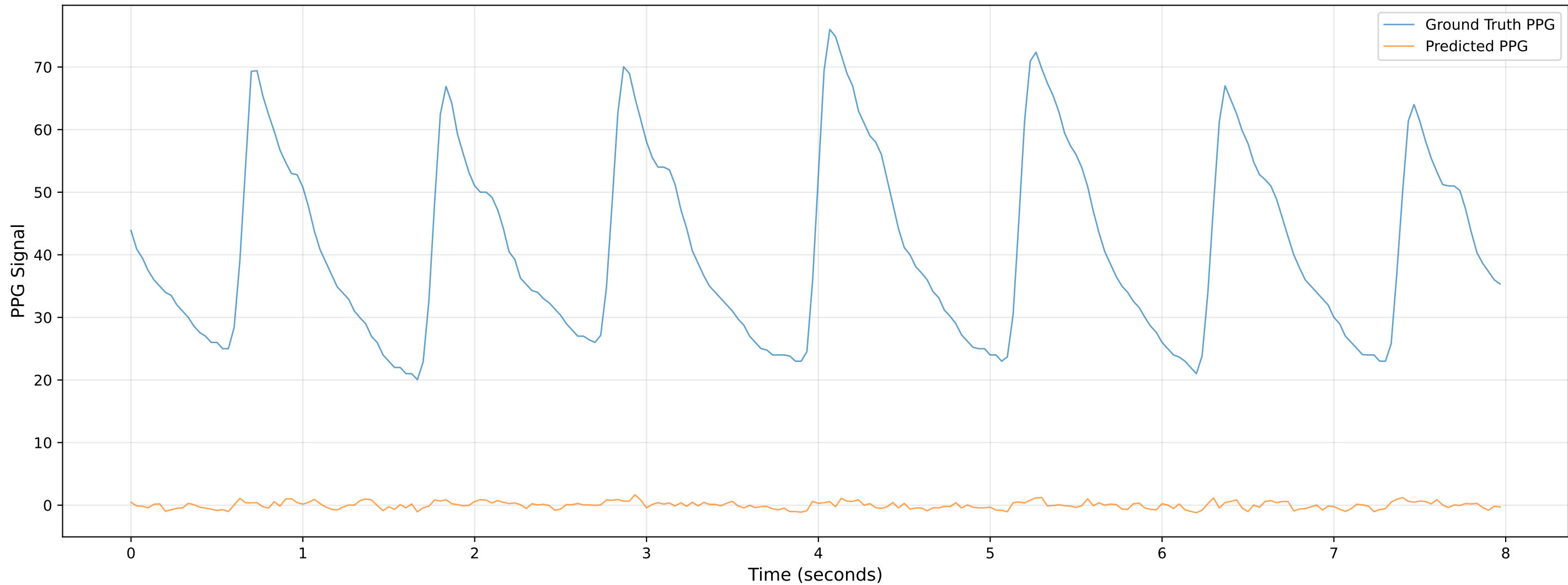
Video 301 - Chunk 7 - Predicted vs Ground Truth PPG
