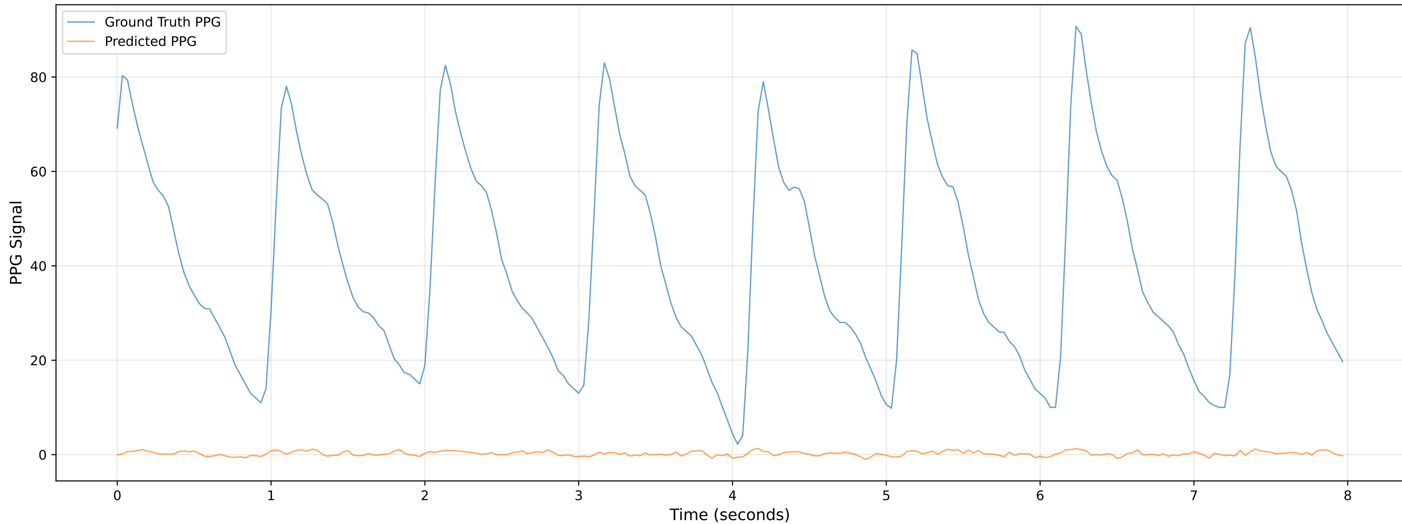
Video 302 - Chunk 7 - Predicted vs Ground Truth PPG
