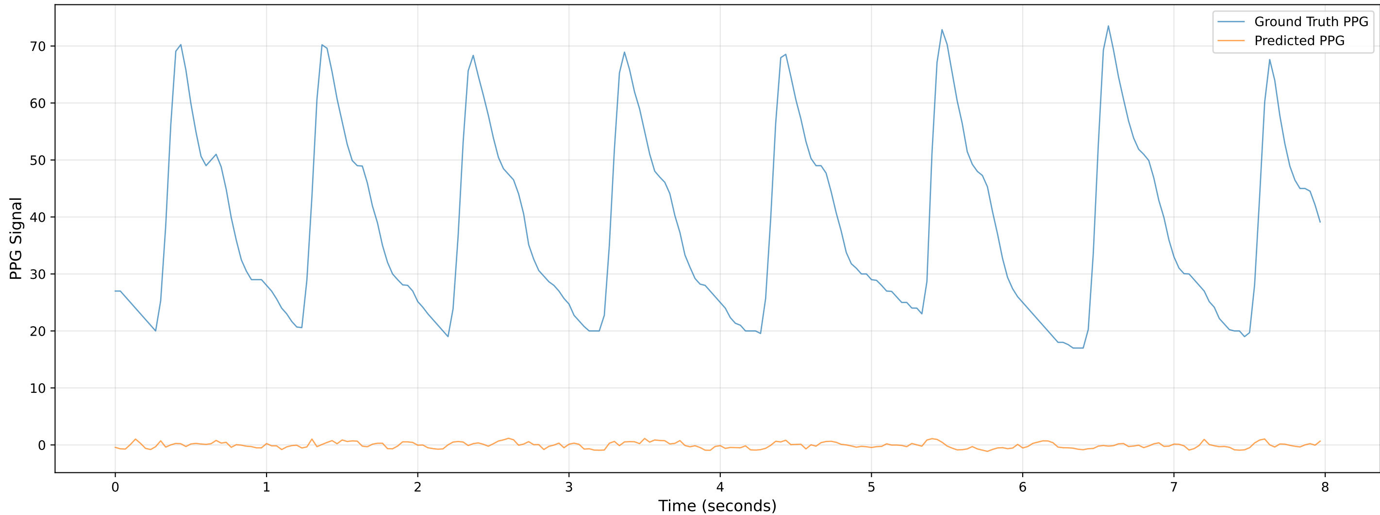
Video 303 - Chunk 0 - Predicted vs Ground Truth PPG
