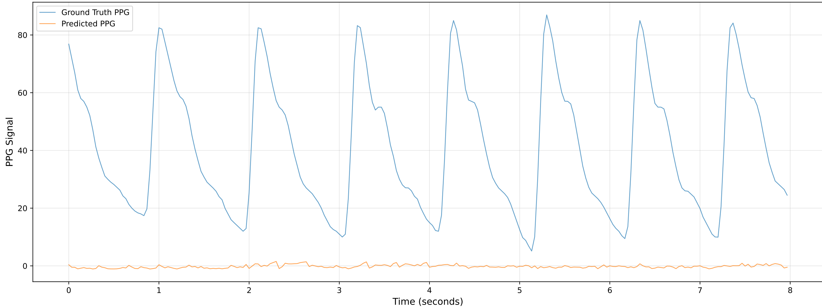
Video 303 - Chunk 5 - Predicted vs Ground Truth PPG
