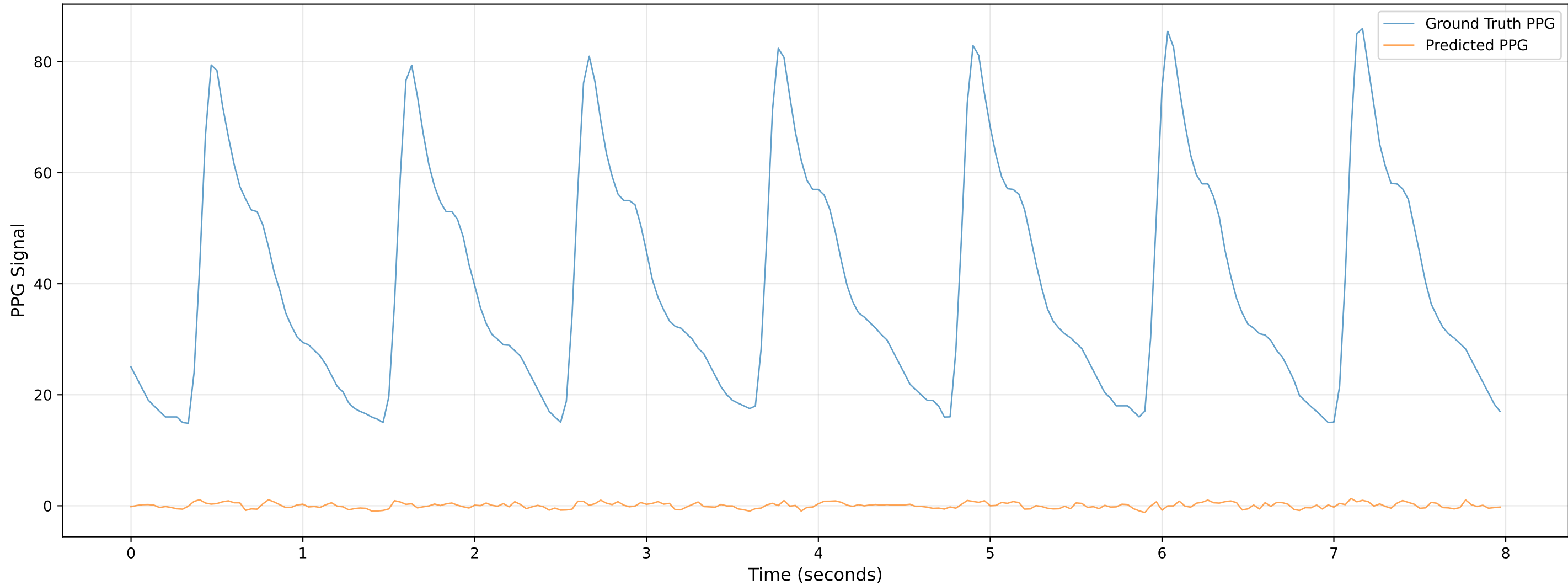
Video 305 - Chunk 0 - Predicted vs Ground Truth PPG
