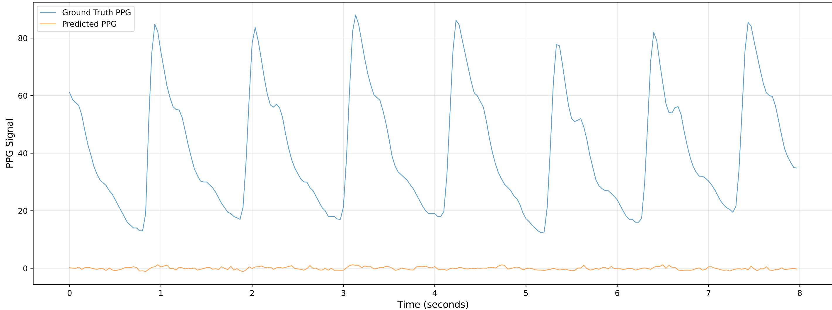
Video 306 - Chunk 5 - Predicted vs Ground Truth PPG
