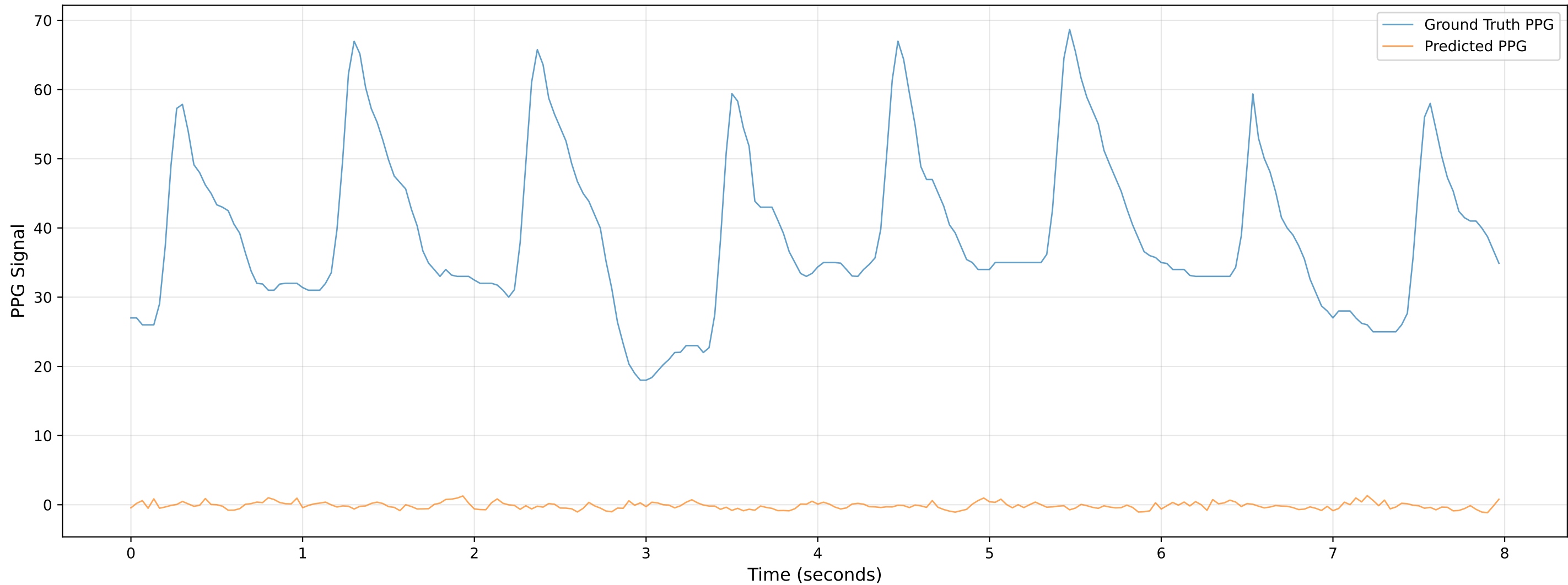
Video 401 - Chunk 2 - Predicted vs Ground Truth PPG
