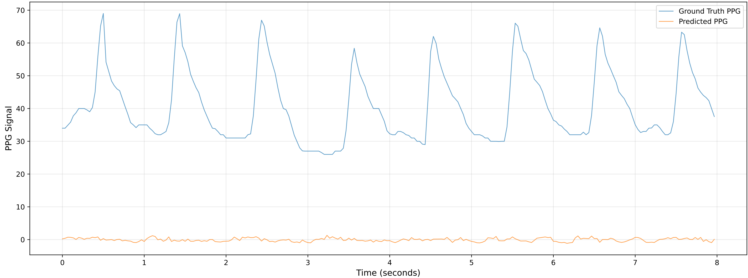
Video 401 - Chunk 3 - Predicted vs Ground Truth PPG
