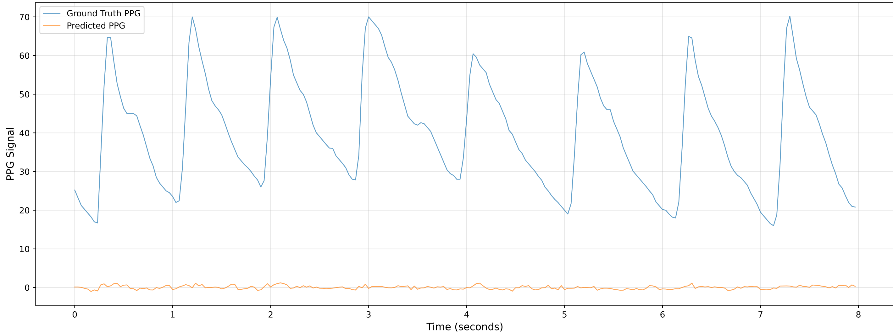
Video 402 - Chunk 2 - Predicted vs Ground Truth PPG
