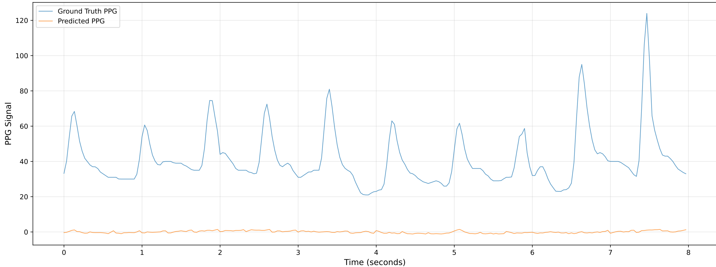
Video 404 - Chunk 4 - Predicted vs Ground Truth PPG
