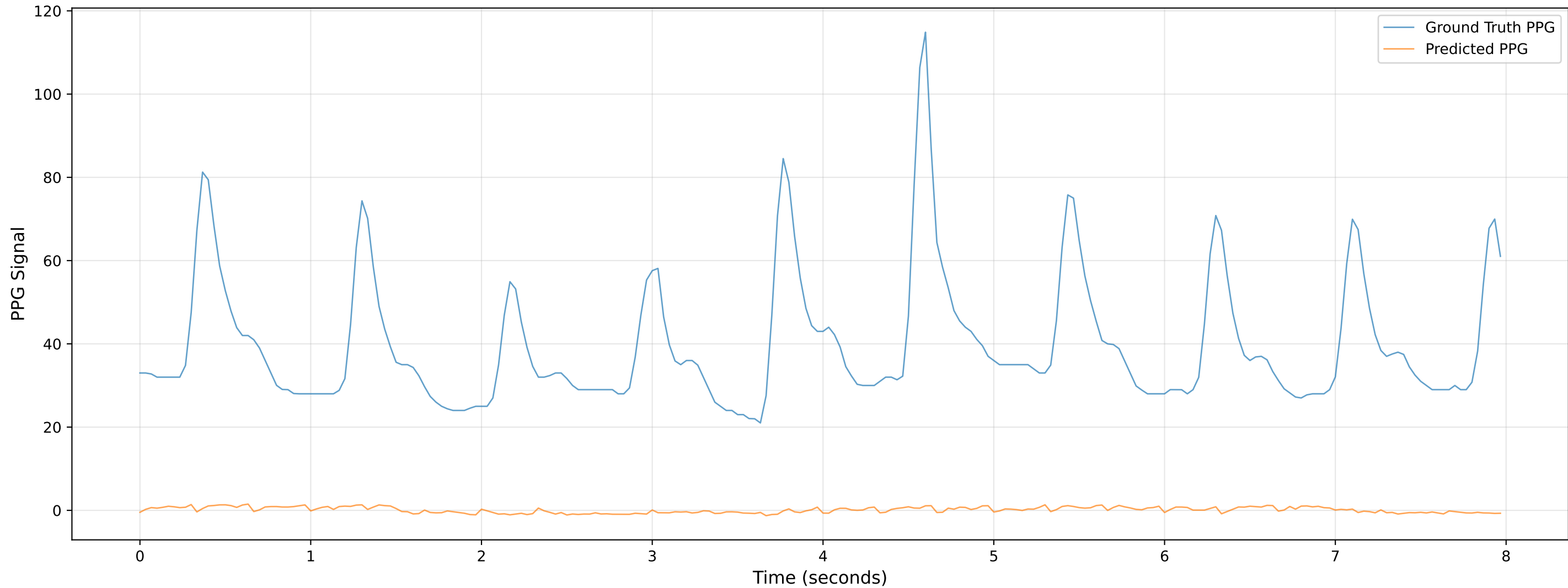
Video 404 - Chunk 5 - Predicted vs Ground Truth PPG
