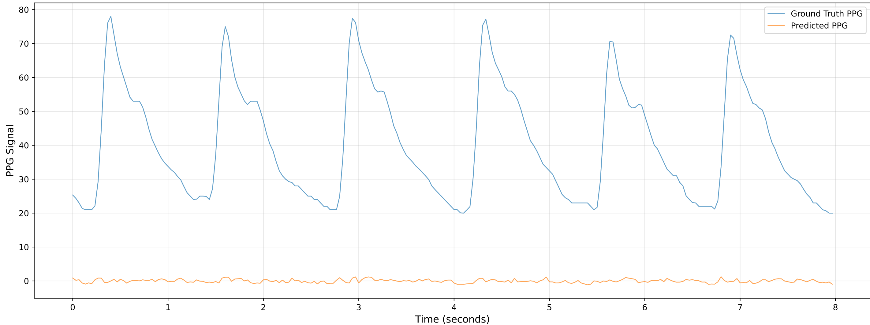
Video 501 - Chunk 6 - Predicted vs Ground Truth PPG
