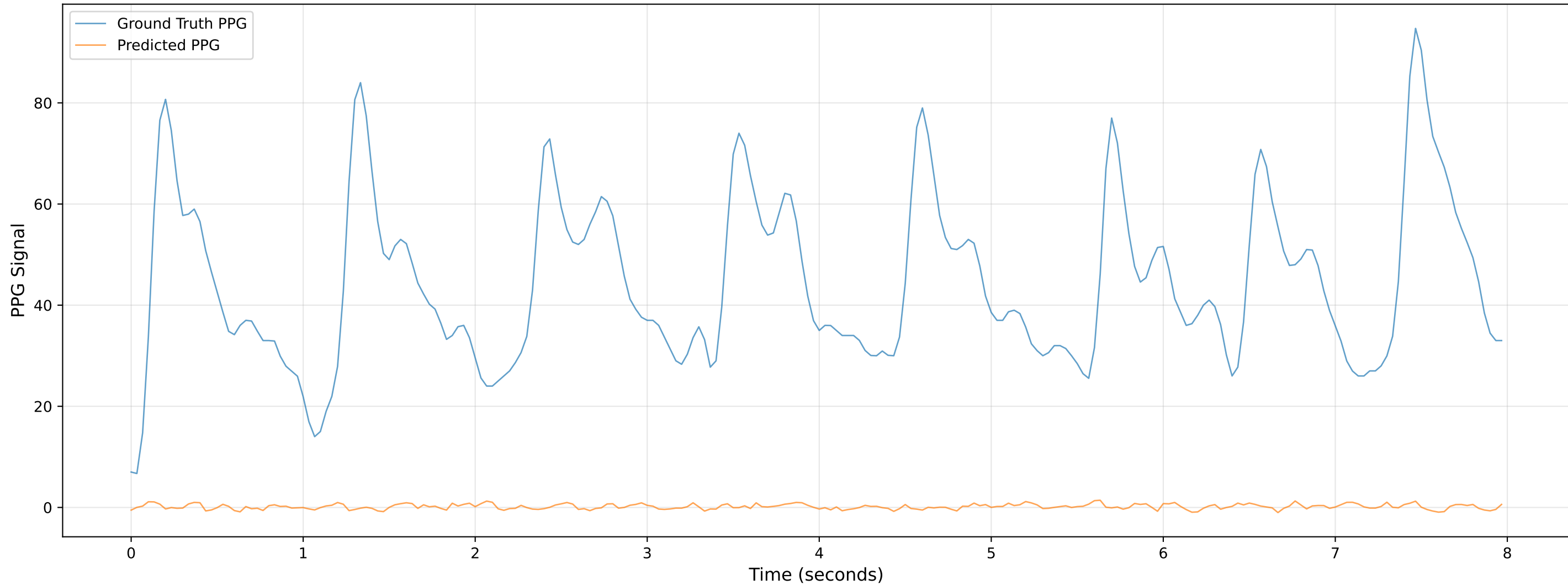
Video 502 - Chunk 1 - Predicted vs Ground Truth PPG
