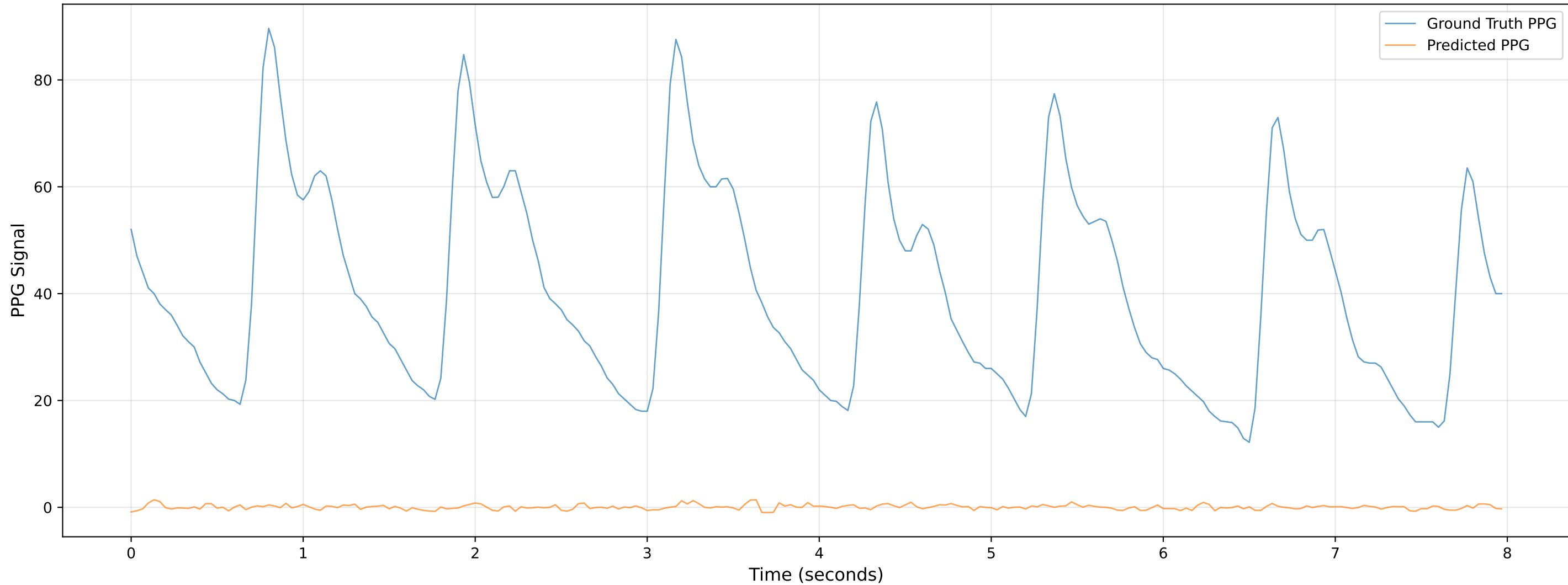
Video 503 - Chunk 0 - Predicted vs Ground Truth PPG
