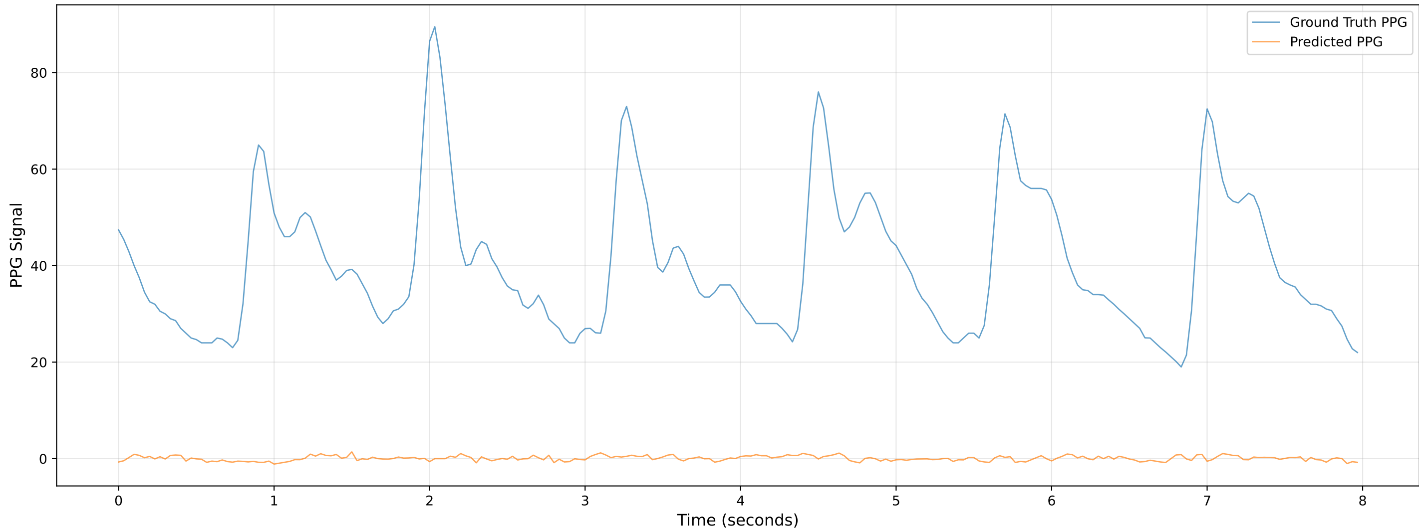
Video 505 - Chunk 1 - Predicted vs Ground Truth PPG
